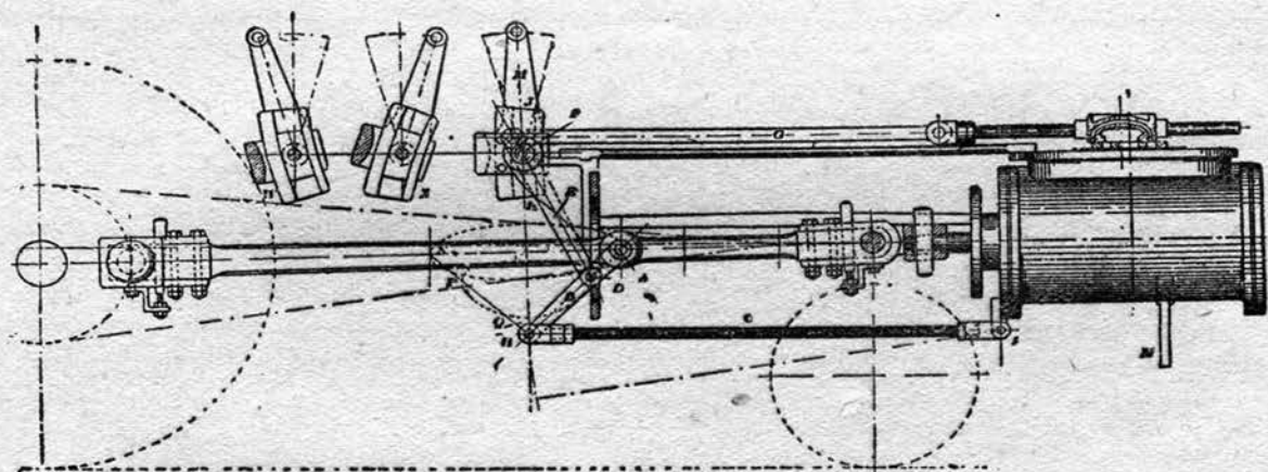
The Joy Valve Gear, Perfected in 1879 by an Englishman Named David Joy. Lever E is Connected to the Vibrating Link B, and Thus Transmits Movement to Valve Rod G. The Fulcrum (F) of Rod E is Carried Vertically in Blocks Which Slide in Slots in the Links (JK). The Engine is Reversed by Moving the Valve Slide. Though the Joy Gear Was Fairly Popular in England, It Was Installed on Only a Few American Engines
